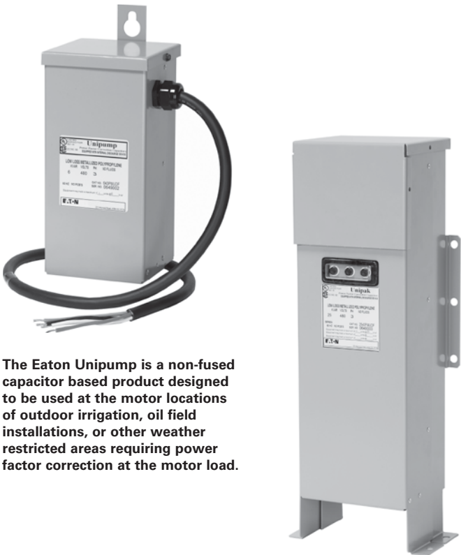
Unipak's are capacitor-based products designed to be used when fixed, static capacitance (wall or floor mounted) is need within parts of your electrical system.
